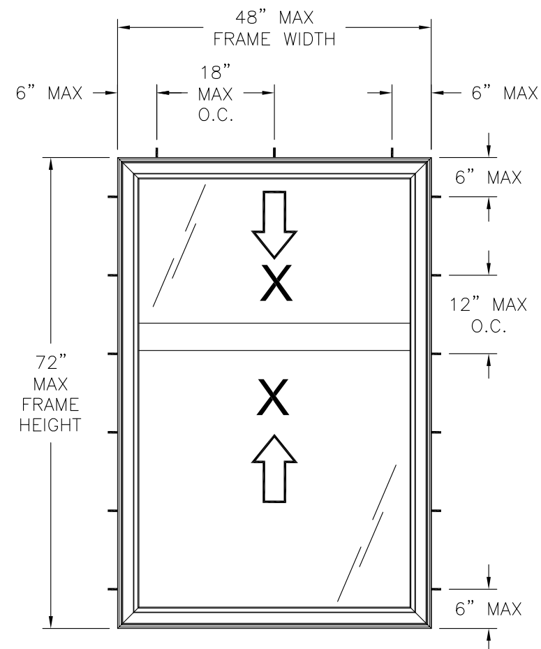
CAMBRIDGE REVERSE ORIEL DOUBLE HUNG EXTERIOR VIEW FRAME INSTALLATION
